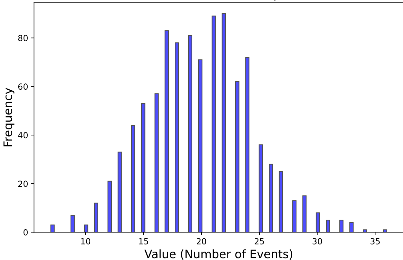
Poisson Distribution (1000 samples, 100 bins)
